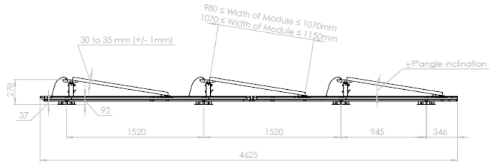
Fig.2 CPX Wave Single Mounting Method-Side View [2]
