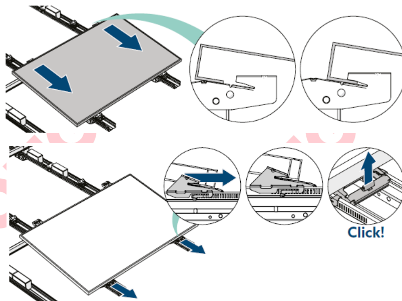
Fig.4 Mounting Locker Method [4]
