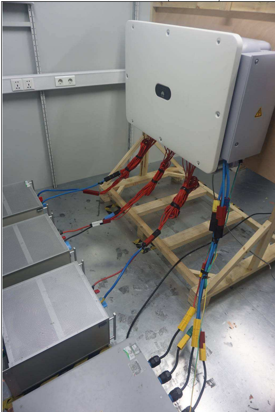
CONDUCTED EMISSION TEST (AC Power Port)
