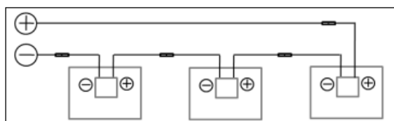
Series Connection
